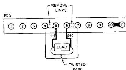
FIG. 3-2 LOAD CONNECTION WITH REMOTE ERROR SENSING
