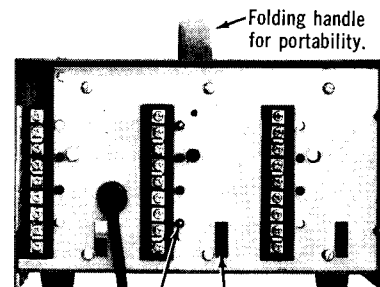
Typical rear view of CA-5, showing Slot provides access to internal coding pins, connectors and line cord. Folding handle for portability.
