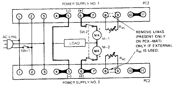
FIG. 3-13 PARALLEL CONNECTION OF PCX-MAT SUPPLIES
