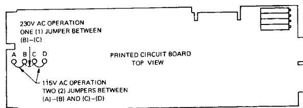
FIG. 2-3 CONVERSION TO 230 V AC LINE OPERATION
