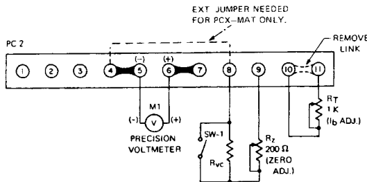
FIG. 3-6 PROGRAMMING RATIO CALIBRATION METHOD #3
