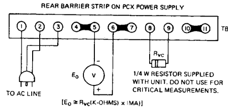
FIG. 2-4 OPERATION CHECK PCX
