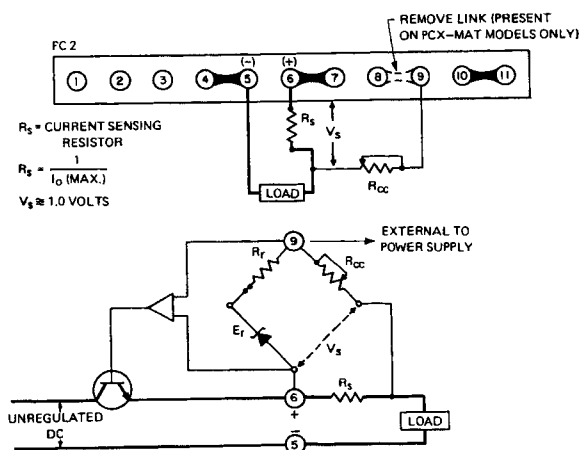
FIG. 3-8 CONNECTIONS FOR CONSTANT CURRENT OPERATION
